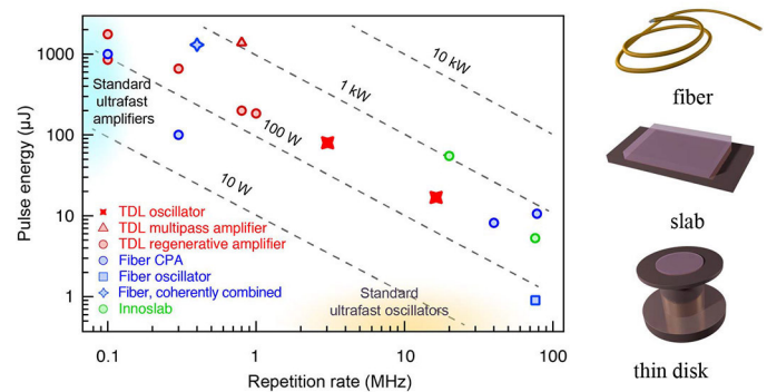
Figure 1. Overview of ultrafast laser sources combining high pulse energy and repetition rate, and illustration of different laser architectures. These optimize heat removal to support very high average power in the kW regime. TDL: Thin disk laser. CPA: Chirped pulse amplification.
