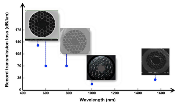
Figure 2. Inhibited coupling (IC) Kagome-type hypocycloid hollow-core photonic crystal fibers (HC-PCF). This type of fiber exhibits extremely low loss in the near-IR-visible spectral range. Record values are 17 decibels (dB)/km at around 1 \mu m, and 70dB/km at 780nm and 500–600nm. IC Kagome HC-PCFs exhibit outstanding guidance and delivery properties, low waveguide dispersion, and anomalous group velocity dispersion over a large portion of the transmission bandwidth, making them excellent candidates for pulse compression applications.
